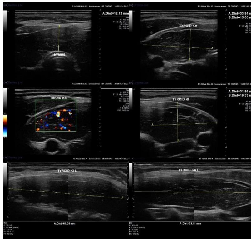
Figure 2. Thyroid ultrasonography
